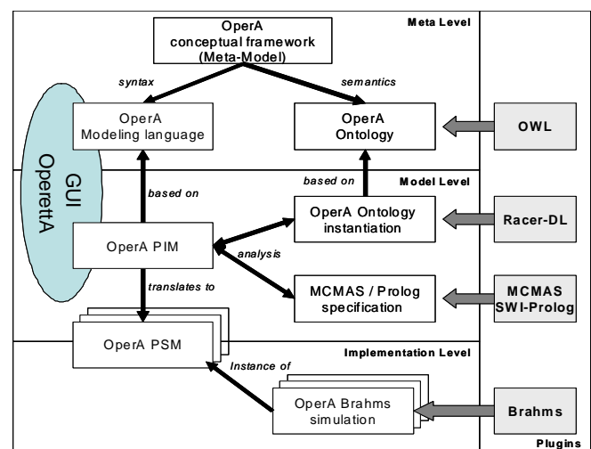
Figure 1 - The OperettA Conceptual Architecture
