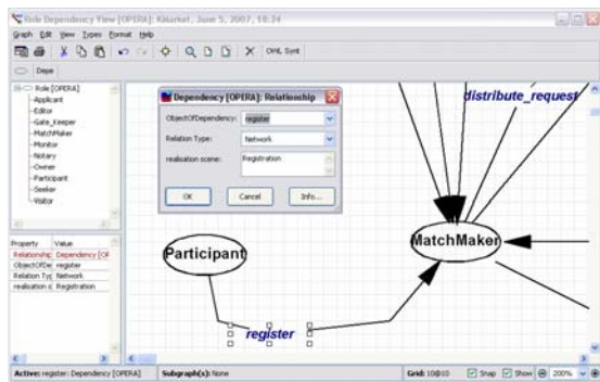
Figure 2: The Operetta Prototype
