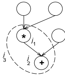
Figure 4: DFG with associated operation labels
