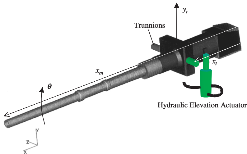
Fig. 2. Rigid-body motion of the barrel due to terrain and actuator forces.
