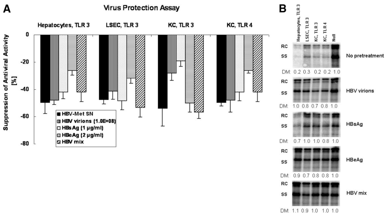
Fig. 2. Purified HBV and recombinant HBV proteins suppress the TLR-induced antiviral activity of parenchymal and nonparenchymal liver cells against EMCV and HBV. Hepatocytes and NPC (KC, LSEC) were stimulated with TLR-3 and TLR-4 ligands for 20 hours (A, B), 6 hours (C), or 2 hours (D) with or without preincubation with supernatants from HBV-Met cells (HBV-Met SN, day 11), HBV virions (1.0E + 08), HBsAg (1 \mu g/mL), HBeAg (2 \mu g/mL), or an HBV mix [HBV virions (1.0E + 08) + HBsAg (1 \mu g/mL) + HBeAg (2 \mu g/mL)] for 24 hours, respectively. Then, the supernatants were (A) used in an antiviral assay (EMCV) or (B) added to differentiated HBV-Met cells with 1:2 dilutions for 2 days. (A) Data are shown as mean antiviral units/mL \pm standard deviation (* P < 0.01 ). (B) HBV replication in HBV-Met cells was analyzed by southern blot. The bands shown correspond to the relaxed circular double-stranded (RC) and single-stranded (SS) HBV DNA replicative intermediates. Densitometric values (DM) are given as ratio sample/untreated control.
