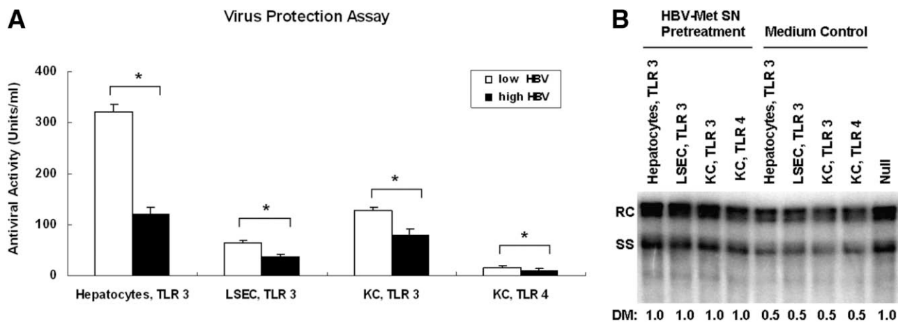
Fig. 1. Supernatants from HBV-Met cells suppress the TLR-induced antiviral activity of parenchymal and nonparenchymal liver cells against EMCV and HBV. Hepatocytes and NPC (KC, LSEC) were stimulated with TLR-3 and TLR-4 ligands for 20 hours with or without preincubation with supernatants from HBV-Met cells (low HBV levels: HBV-Met SN from day 2, containing 8.21 IU/mL HBsAg and 24.14 S/CO reactive HBeAg); high HBV levels: HBV-Met SN from day 11, containing 169.97 IU/mL HBsAg and 119.4 S/CO reactive HBeAg) for 1 day. Then, the supernatants were used (A) in an antiviral assay (EMCV) or (B) added to differentiated HBV-Met cells with 1:2 dilutions for 2 days. In A, data are shown as mean antiviral units/mL \pm SD (* P < 0.01 ). (B) HBV replication in HBV-Met cells was analyzed by southern blot. The bands shown correspond to the relaxed circular double-stranded (RC) and single-stranded (SS) HBV DNA replicative intermediates. Densitometric values (DM) are given as ratio sample/untreated control.
