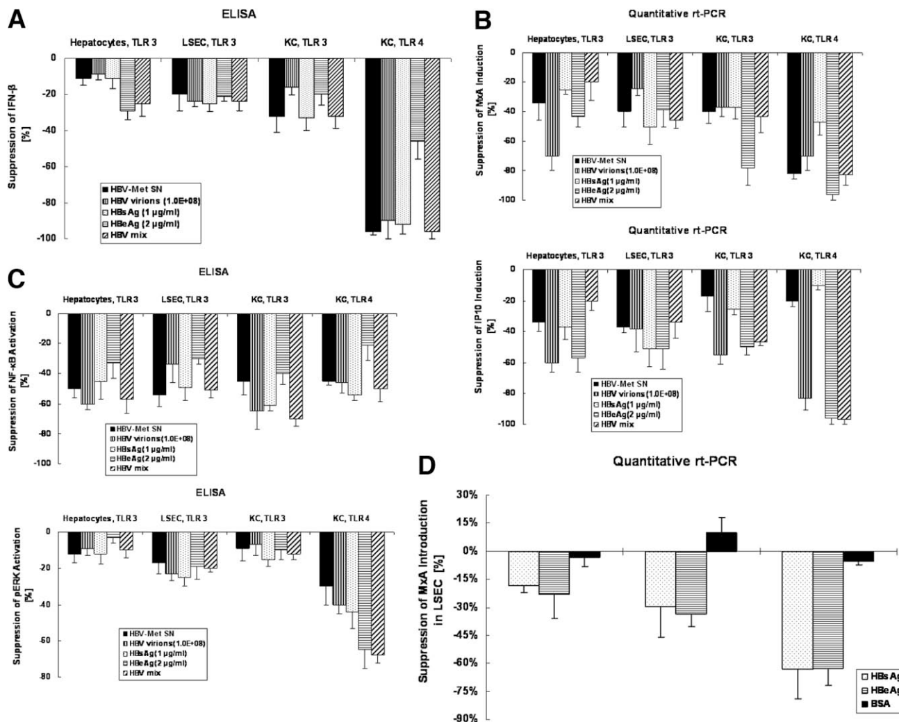
Fig. 3. HBV suppresses TLR-induced IFN- \beta production, ISG expression, and induction of transcription factors in parenchymal and nonparenchymal liver cells. Hepatocytes and NPC (KC, LSEC) were stimulated with TLR-3 and TLR-4 ligands with or without preincubation with supernatants from HBV-Met cells (HBV-Met SN, day 11), HBV virions (1.0E + 08), HBSAg (1 \mu g/mL), HBeAg (2 \mu g/mL), or an HBV mix [HBV virions (1.0E + 08) + HBSAg (1 \mu g/mL) + HBeAg (2 \mu g/mL)] for 24 hours, respectively. Then, (A) supernatants were harvested after 6 hours and assayed for the presence of IFN- \beta by enzyme-linked immunosorbent assay. (B) Total RNA was extracted after 6 hours, and expression of MxA and IP10 was analyzed by quantitative RT-PCR. (C) After 2 hours, total protein was isolated and assayed for the presence of activated ERK \frac{1}{2} , and nuclear protein was isolated to analyze the amount of translocated NF- \kappa B (p65) by enzyme-linked immunosorbent assay. (D) LSECs were stimulated with TLR-3 ligands with or without preincubation with different concentrations of HBSAg and HBeAg. Total RNA was extracted after 6 hours, and expression of MxA was analyzed by quantitative RT-PCR. Data are shown as mean \pm standard deviation suppression of the TLR response of hepatocytes and NPC induced by pretreatment with HBV or HBV proteins.
