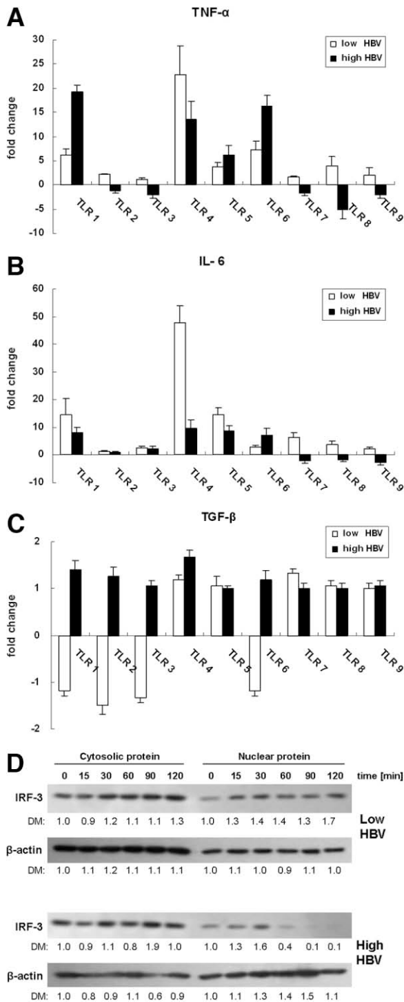
Fig. 4. Modulation of TLR responses in HBV-Met cells by HBV. Undifferentiated (day 2, low HBV levels) and differentiated HBV-Met cells (day 11, high HBV levels) were stimulated with TLR 1-9 ligands for 6 hours. Total RNA was extracted, and expression of TNF- \alpha (A), IL-6 (B), and TGF- \beta (C) was analyzed by quantitative RT-PCR. Data are shown as fold change compared with unstimulated cells. (D) Cytosolic proteins and nuclear proteins were subjected to sodium dodecyl sulfate polyacrylamide gel electrophoresis followed by immunoblotting using anti-mouse IRF-3 antibodies. Densitometric values (DM) are given as ratio sample/untreated control.
