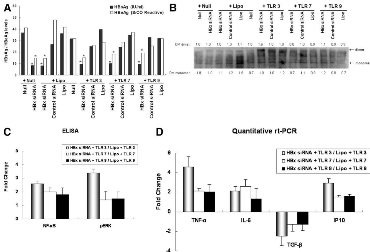
Fig. 5. Integrated HBV down-regulates the TLR response of hepatocytes. HBV-Met cells were transfected with HBx siRNA, green fluorescent protein siRNA (control siRNA), or lipofectamine 2000 on day 1 followed by stimulation with TLR-3, TLR-7, and TLR-9 ligands for 20 hours (A), 2 hours (B), 2 hours (C), or 6 hours (D) 7 days posttransfection. (A) HBsAg and HBeAg levels in cell culture medium were analyzed by chemiluminescent microparticle immunoassay. Significant levels of suppression ( P < 0.05 ) are indicated by the asterisk. (B) The cell extracts were subjected to native polyacrylamide gel electrophoresis (PAGE) followed by immunoblotting using anti-mouse IRF-3 antibodies. Densitometric values (DM) are given as ratio sample/untreated control. (C) Total or nuclear protein was isolated, and the amount of NF- \kappa B and pERK was detected by enzyme-linked immunosorbent assay. (D) Total RNA was extracted, and expression of cytokines TNF- \alpha , IL-6, TGF- \beta , and antiviral genes IP10 were analyzed by quantitative RT-PCR. Data are shown as fold change of siRNA pretreatment compared with lipofectamine-treated controls.
