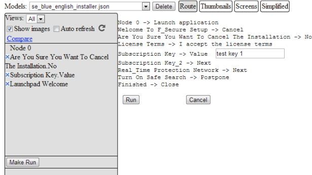
Fig. 3. Defining input values for a test case with Murphy Web UI.
