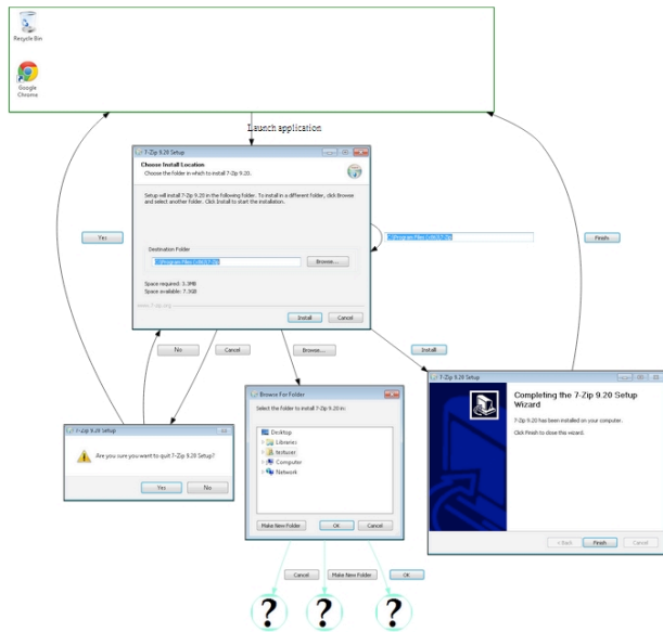
Fig. 2. A simple example of a GUI model extracted by Murphy.
