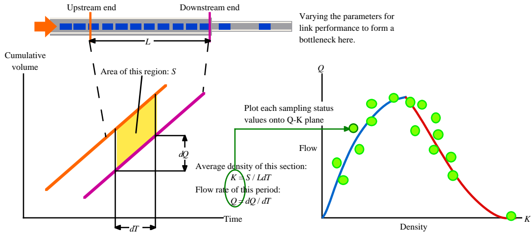
Fig.3: The verification step of flow characteristic of C-F type simulation model.
