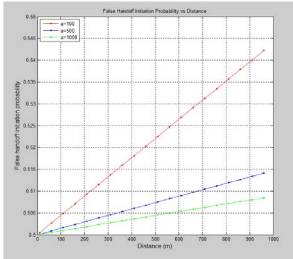
Figure-6. Relationship between false handoff probability and distance with different value of cell size.
