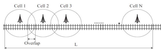
Figure-1. Wireless coverage along railway.
