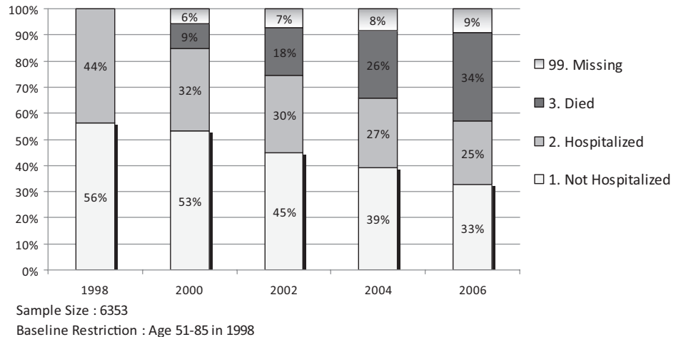
FIGURE 1. Sample distribution of outcome variables.
