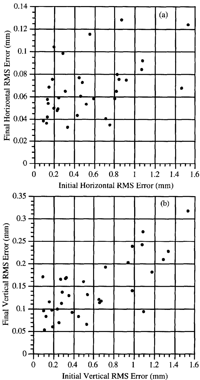
Figure 2. Final beam position error versus Initial beam position error for (a) horizontal and (b) vertical plane for one iteration of the beam steering algorithm.
