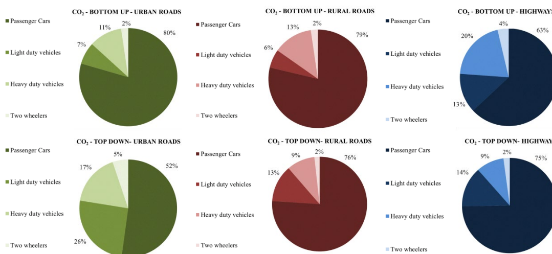
Figure 22. Apportionment among vehicle types of CO 2 emissions assigned to urban roads, rural roads and highways in bottom-up and top-down approaches.
