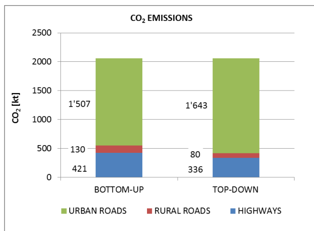
Figure 21. Apportionment among road types of CO 2 emissions in bottom-up and top down approaches.
