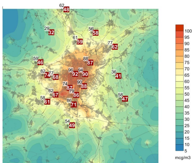
Figure 23. Average NO 2 concentration field of January and February 2008. Simulated values in red and monitoring data in black
