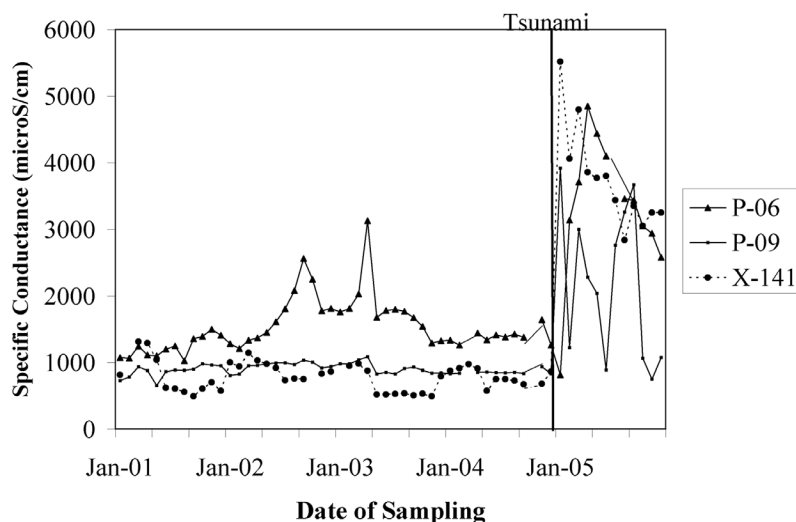
Figure 2. Specific conductance of groundwater from three tube wells in Kaggola, Sri Lanka. These wells were inundated to various degrees by the tsunami; however, it is not believed that significant volumes of seawater entered these wells directly during overtopping. All wells show a rapid rise in specific conductance following the tsunami and have not yet returned to background levels.
