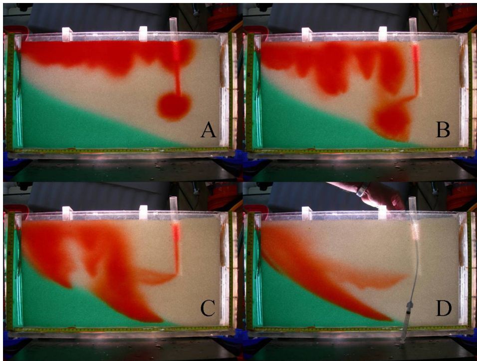
Figure 3. Physical model of tsunami injection and infiltration into a shallow coastal sandy aquifer at (a) 2, (b) 5, (c) 11, and (d) 19 min. The pre-tsunami seawater wedge is dyed green, and the pre-tsunami fresh water flowing from right to left is light brown. Infiltrated tsunami water, dyed red, is injected across the top of the aquifer. Tsunami water is also immediately injected into the aquifer through the open borehole. Dense seawater quickly develops into plumes that reach the preexisting seawater wedge.
