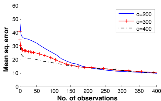
Figure 2: Error measuring difference between a robot’s cost estimation and that of a human; parameter o specifies the number of obstacles.
