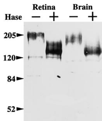
FIGURE 5. Immunoblotting for N-syndecan. In the retinal homogenate before treatment (-) with heparitinase I (Hase), a broad band that corresponded to a molecular mass of approximately 200 kDa was detected. After treatment (+), the broad band became more distinct with a molecular mass of 140 kDa. In addition, a heparitinase-resistant immunopositive band was weakly detected at 120 kDa. In the brain homogenate before treatment with heparitinase I, a broad band was detected at approximately 200 kDa, whereas, after treatment, a 140 kDa-band was observed. The positions of the molecular mass markers are indicated in kilodaltons.
