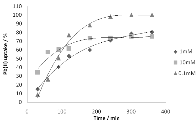
Figure 3 Lead uptake against time for Ca-Alg films in Pb(II) solutions with different concentration
