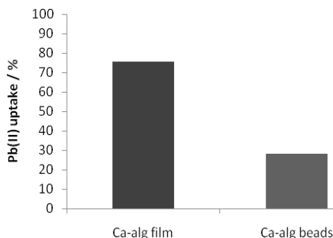
Figure 4. Lead uptake percentage for calcium alginate films and beads after 360 minutes
