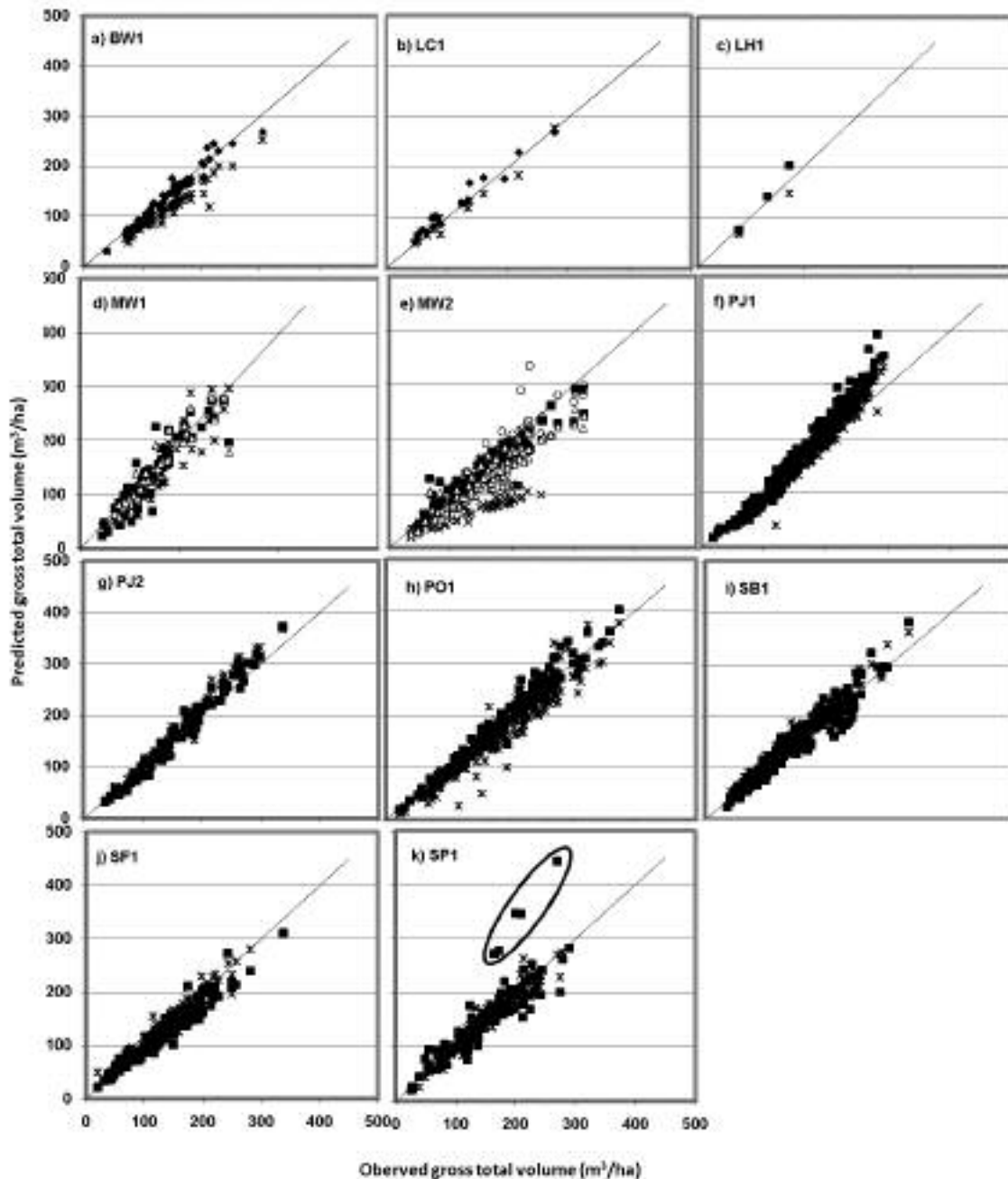
Fig. 2. Gross total volume predictions are plotted against the observed volume for the validation data set by forest unit. ■: forest unit predictions, ×: leading species predictions, and Δ: for the leading species within forest unit for the MW1 and MW2 forest units. In (e) MW2, softwood predictions using the forest unit approach are given by ○. The circled predictions in (k) SP1 have jack pine as the leading species despite being classified as SP1.
