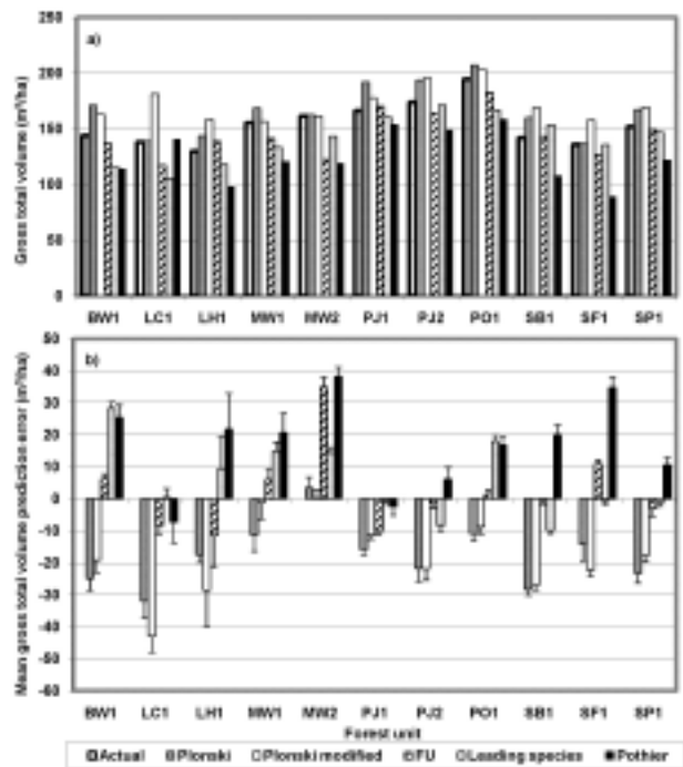
Fig. 5. Mean actual and predicted gross total volume (a) and the mean prediction error (bias) and the standard error of the prediction errors are given by forest unit (b) for the validation data. Gross total volume is not available for the northeast regional yield curves. In contrast to the rest of the models, the Pothier predictions errors are based on gross total volumes for trees >9 cm in diameter at breast height and are compared to the actual volume associated with trees that size. A positive prediction error indicates underprediction.
