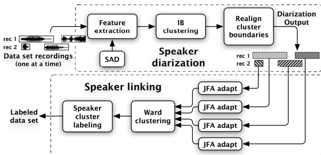
Figure 1: Block diagram of the speaker diarization and linking system.
