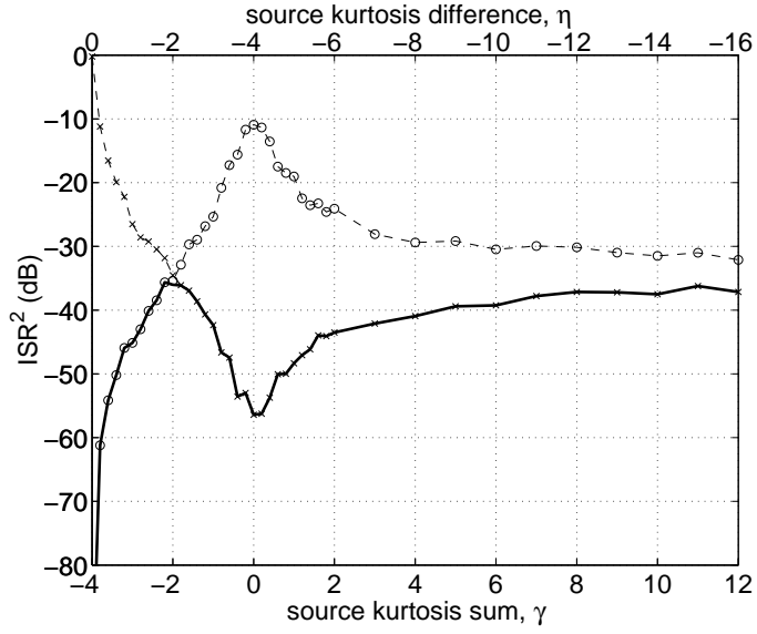
Figure 1: Performance of EML, AEML and combEML estimators against source kurtosis. PRBS sources, \kappa_{40}^x = -2 , T = 5 \times 10^3 samples/signal, 100 Monte Carlo runs.
