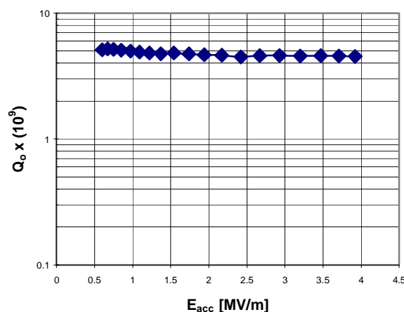
Figure 2, first results for the Horizontal Cryostat cavity test.
