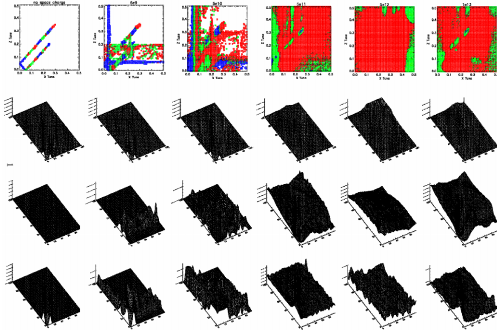
Figure 6: Top row: The average chaos of the bin red is chaotic, green is weakly chaotic, blue is regular. Second row: Shows the distribution in tune-space. Third row: The average space-charge kick. Fourth row: The average radius.
