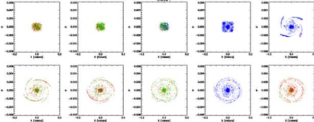
Figure 3: Slices at turn 100-1000 in 100 turn increments. Red points are chaotic, green points are weakly chaotic, and blue points are regular. These plots show the 5 \times 10^{11} regime.
