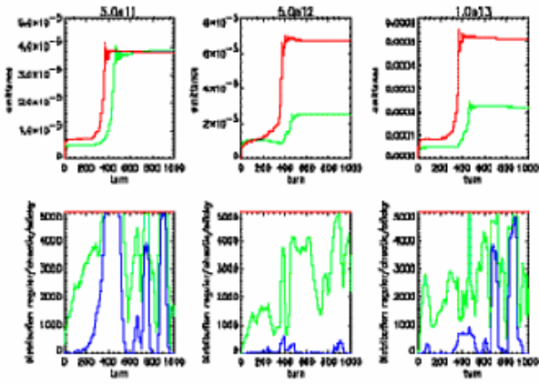
Figure 2: Plots of emittance and relative chaos. In the top row red denotes emittance in the z dimension, green is emittance in the x dimension. In the bottom row blue denotes regular orbits, green denotes weakly chaotic orbits + regular orbits, and red is the sum of all three.
