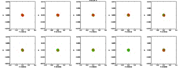
Figure 4: Slices at turn 100-1000 in 100 turn increments. Red points are chaotic, green points are weakly chaotic, and blue points are regular. These plots show the 5 \times 10^{12} regime
