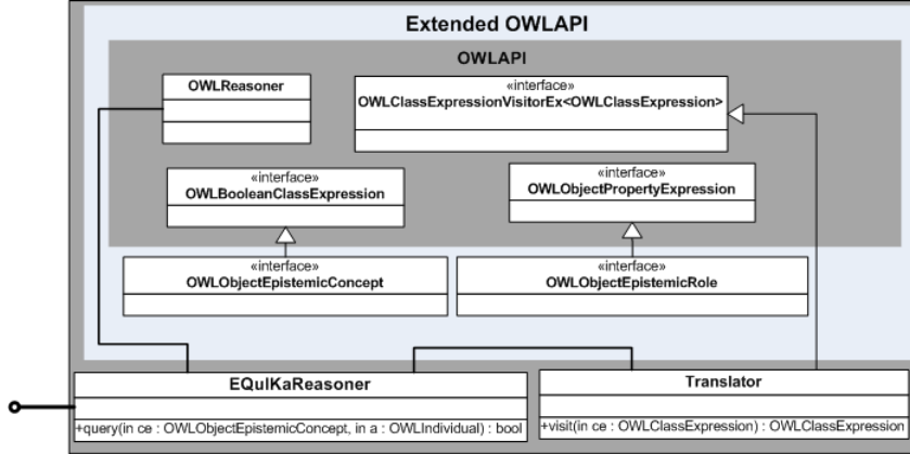
Fig. 2. The EquiKa -system extending the OWL-API
