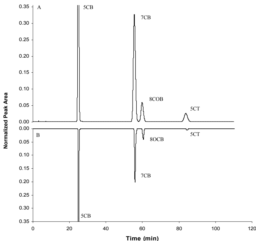
Figure 4: HPLC chromatograms of E7: A- mixture commercially available and B- mixture from VLE sample (experiment at 40 °C and 13.59 MPa). The peaks were normalized by the 5CB peak and were represented in this scale for a better viewing of the smaller peaks.
