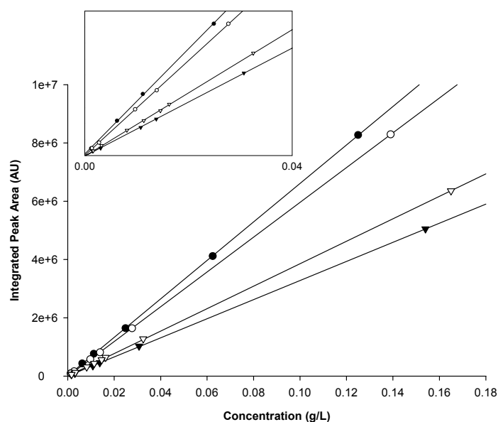
Figure 3: Calibration curves (integrated HPLC peak area vs. concentration) for E7 constituents (5CB-full circles: y = 6.60 \times 10^7 x + 1.08 \times 10^3 ; 7CB-open circles: y = 5.97 \times 10^7 x - 6.29 \times 10^3 ; 8OCB-full triangles: y = 3.28 \times 10^7 x + 2.57 \times 10^3 and 5CT-open triangles: y = 3.85 \times 10^7 x + 3.85 \times 10^3 . All r^2 = 0.9999 or better). The inset amplifies the region of lowest concentrations.
