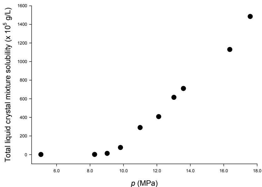
Figure 6: Total liquid crystal mixture solubility as a function of pressure in supercritical CO 2 at 313.15K.
