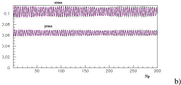
Fig.4: The same of fig.3, but for \sigma/\sigma_0=0.29 , with initial K-V beam particle distribution.
