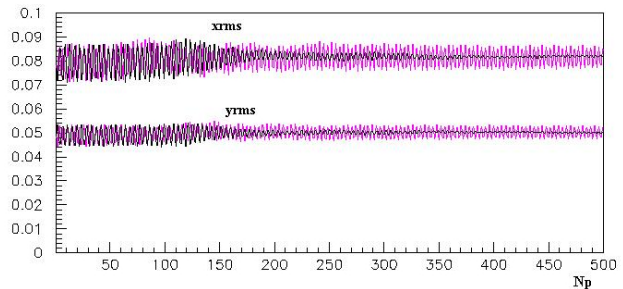
Fig.1: x and y rms-envelope oscillations for even (magenta-line) and odd mismatched beam (black-line), with initial KV distribution, along the FODO channel.
