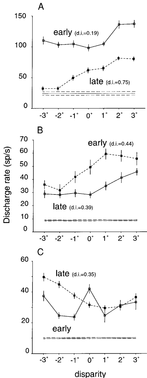
FIG. 2. Disparity tuning of FEF neurons. Examples from 3 neurons. Mean and SE discharge rate are shown at each disparity value tested. \square , activity relative to the early visual response; \blacksquare , activity relative to the late visual response. Bottom lines indicate mean and SE of the control activity. Figure 2A shows the same neuron as in Fig. 1, B and C. Disparity indices (d.i.) are shown for each curve.
