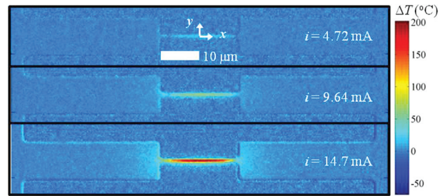
Fig. 5 2D temperature difference measurement during quasi-steady increase of Joule heating in the structure under \lambda_{\text{LED}} = 535 nm
