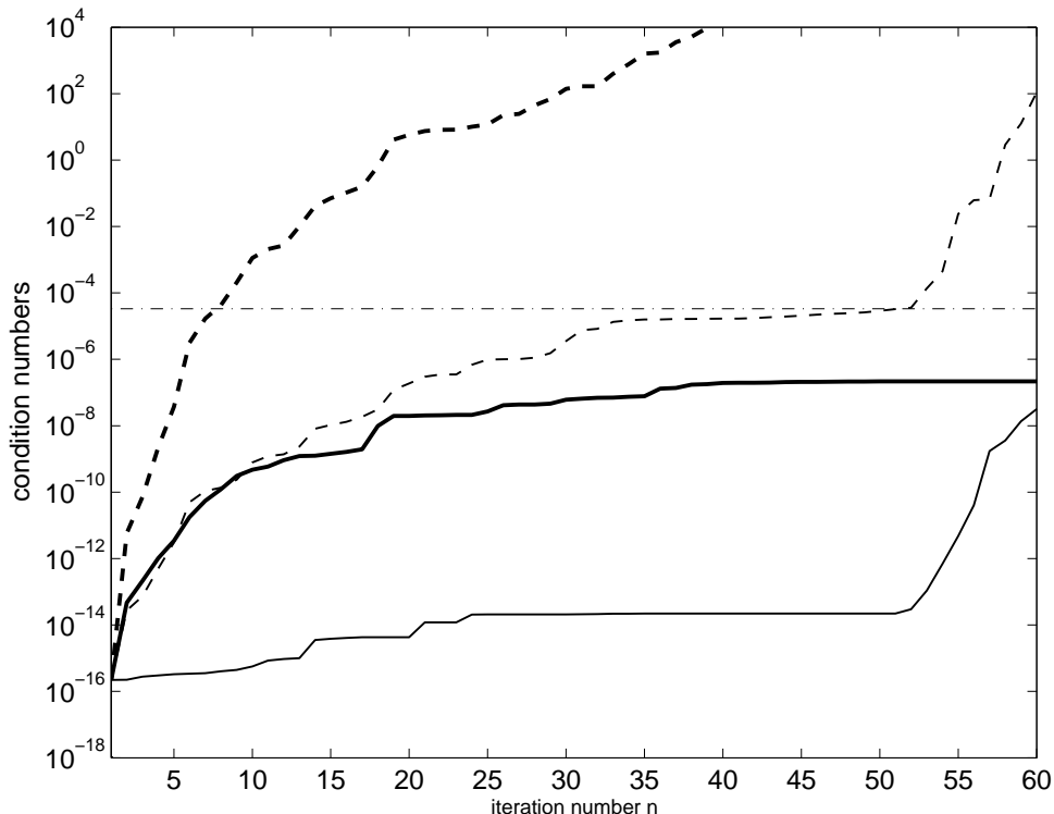
FIG. 3.3. The test problem FS1836, condition numbers multiplied by unit roundoff u : \kappa(A) (dash-dotted line); \kappa(Z_n) (thick solid line) and \kappa(U_n) (thick dashed line) for Z_n = \left[ \frac{r_0}{\|r_0\|}, V_{n-1} \right] ; \kappa(Z_n) (thin solid line) and \kappa(U_n) (thin dashed line) for Z_n = \tilde{R}_n .
