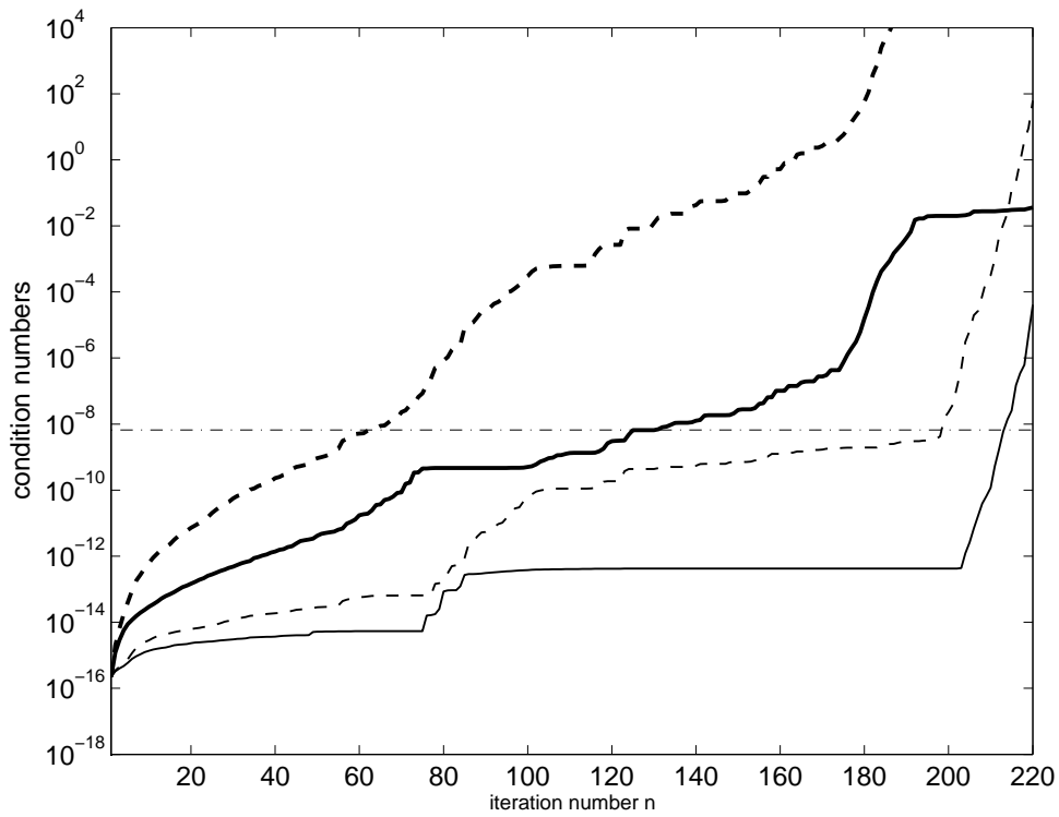
FIG. 3.6. The test problem STEAM1 , condition numbers multiplied by unit roundoff u : \kappa(A) (dash-dotted line); \kappa(Z_n) (thick solid line) and \kappa(U_n) (thick dashed line) for Z_n = \begin{bmatrix} \frac{r_0}{\|r_0\|} \\ V_{n-1} \end{bmatrix} ; \kappa(Z_n) (thin solid line) and \kappa(U_n) (thin dashed line) for Z_n = \tilde{R}_n .
