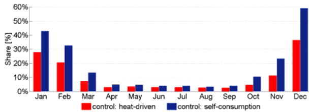
Figure 3: Monthly analysis of self-consumption for an exemplary household (left bar: heat-driven, right bar: control for a maximized self-consumption)
