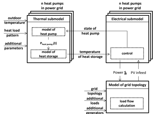
Figure 2: Basic functionality of the electrical-thermal model applied within this paper
