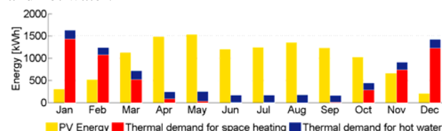
Figure 1: Electric energy production by a PV unit and thermal energy demand for space heating and hot water for an exemplary household
