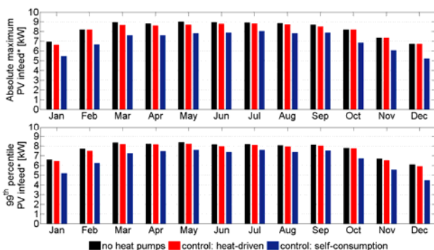
Figure 4: Absolute maxima and 99 th percentiles of the sum of the PV power and the power demand of the heat pump (*: PV infeed without remaining load of household)
