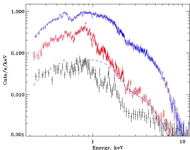
Fig. 7. EPIC MOS1 spectra collected from different regions of the M 31 bulge. Blue crosses represent the sum of 44 bright sources located within 5' from the centre; the violet line is a fit of this spectrum with a single power-law model. The spectrum of unresolved emission is shown by red diamonds; the blue dashed line shows contribution of a power-law component with the same slope as the top curve. The need for an additional thermal plasma component associated with the diffuse bulge emission is clearly seen. The pink solid line is a fit of the unresolved-emission spectrum with a two-component model. Black crosses below show the background, collected in the outer parts of the same MOS chip. All three spectra are normalised to the same area. The two upper spectra have been background-subtracted using the bottom background spectrum scaled to the appropriate area. See the text for details of the analysis and model parameters
