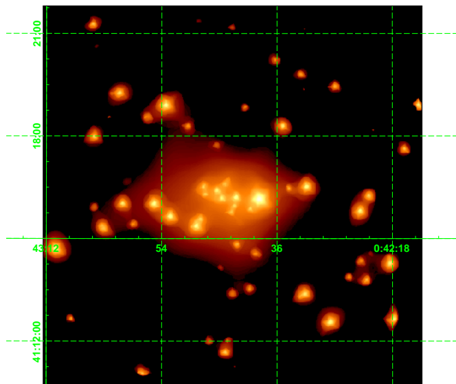
Fig. 6. Wavelet-deconvolved EPIC MOS1 image of the central 10' of M 31, showing diffuse emission as well as numerous point sources
