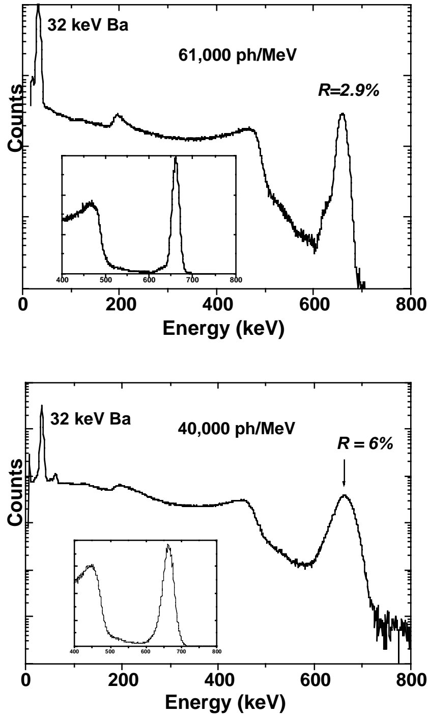
Figure 3: Pulse height spectra of LaB 3 :Ce (upper) and NaI:Tl (lower) when excited by 662 keV gamma rays. The ordinates are on a logarithmic scale — the inset plots show the same data on a linear scale.
