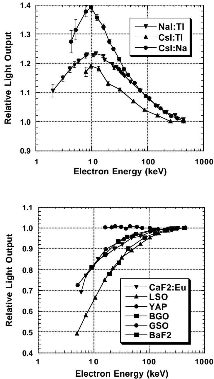
Figure 2: Electron energy response (relative light output, normalized to the value at 662 keV, as a function of electron energy) for various alkali halide (upper) and non-alkali halide (lower) scintillators. The response of an ideal material would be independent of electron energy.
