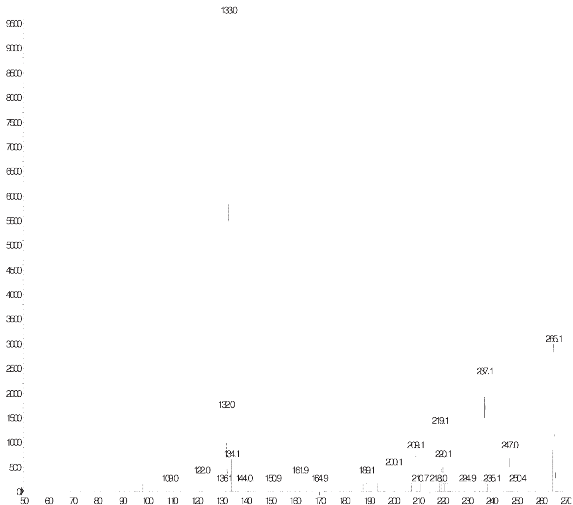
FIG. 5. MS/MS spectrum of protonated M5+M6, M7 (M8) at m/z 265, and the proposed origin of key product ions.
