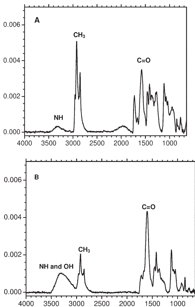
FIG. 8. IR absorption spectra of meisoindigo metabolites at m/z 279 (A) and m/z 295 (B).
