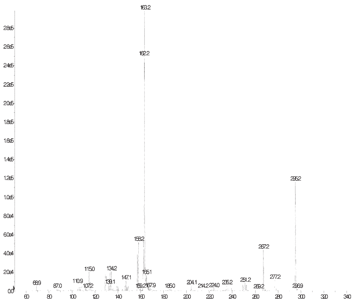
Fig. 6. MS/MS spectrum of protonated M9, M11, M13, and M15 at m/z 295 and the proposed origin of key product ions.
