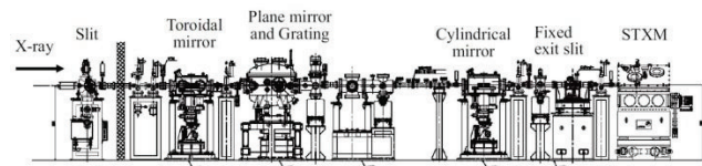
Figure 4: Schematic image of the optical system of BL4U.
