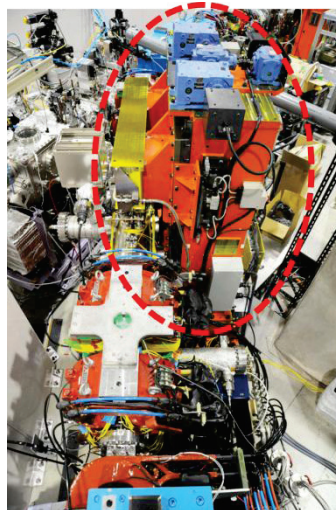
Figure 3: New in-vacuum undulator for BL4U STXM beam-line.
