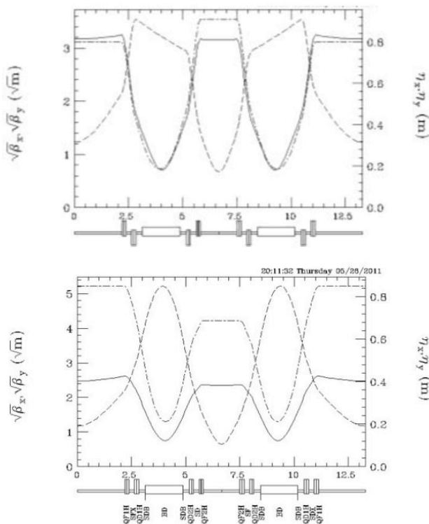
Figure 2: Optics of UVSOR-II (up), and III (down). The betatron functions in the horizontal and vertical plane (solid and dashed line) and the dispersion function (chain line).
