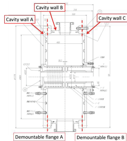
Figure 6: main cavity of the ring.
