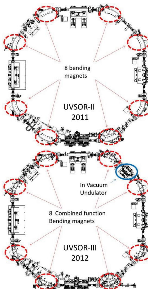
Figure 1: Layout of UVSOR-II (up) and UVSOR-III (down).
