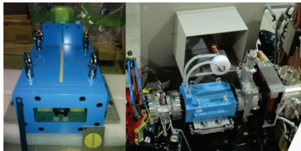
Figure 5: Photo of the pulse sextupole magnet.
