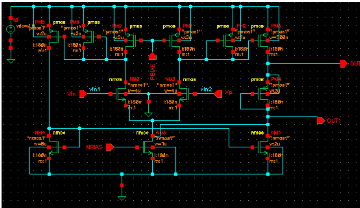
Fig. 5: Operational amplifier
