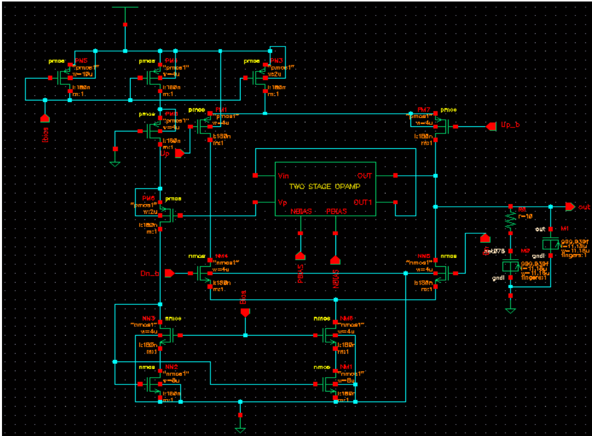
Fig. 4: Charge pump
