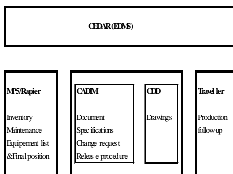
Figure 1: Overview of CERN EDMS.
