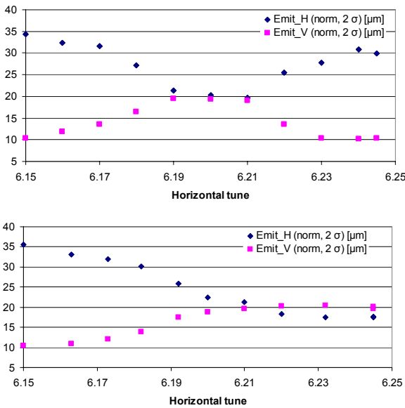
FIGURE 2. Measured intensity-dependent emittance transfer in 2003 for Q_y = 6.21 (upper) in the static case (constant horizontal tune from injection to the measurement point), (lower) in the dynamic case (the horizontal tune was changed linearly from 6.15 to 6.25 in 100 ms).
