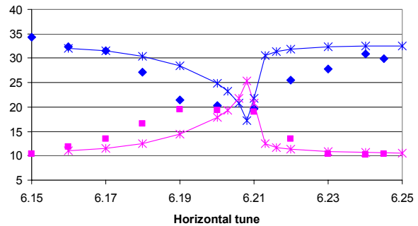
FIGURE 3. Measured (dots, see Fig. 2) and simulated (full line) intensity-dependent emittance transfer in the static case.
