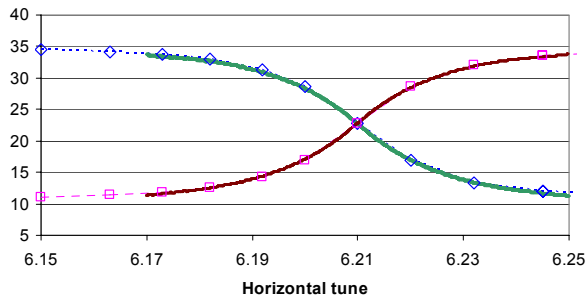
FIGURE 4. 3D simulation results (IMPACT code) in the case where the synchrotron period is much larger than the crossing time (full line), and fit (dotted line), using the numerical values of the measured case (see Fig. 2).
