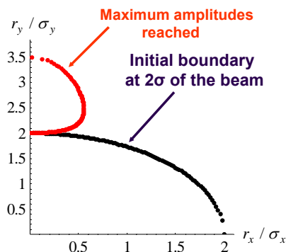
FIGURE 1. Initial and maximum transverse amplitudes in the “Montague stop-band” in an example case with PS parameters close to the experimental conditions (see measurements section).
