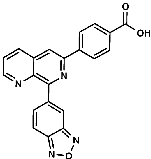
Fig. 1. Structure of NVP-ABE171.
