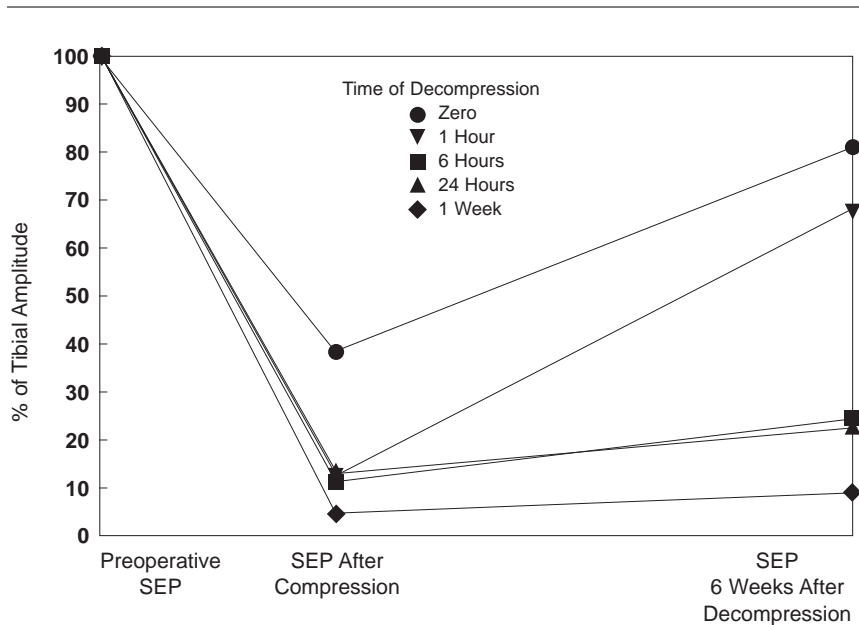
Fig. 2 Somatosensory evoked potential (SEP) recovery after decompression of experimental spinal cord injury in 30 dogs. Note the mean deterioration of the amplitude of posterior tibial SEPs, compared with preoperative values, after compression of the spinal cord and the subsequent recovery in amplitude 6 weeks after decompression. Six weeks after decompression, only the dogs in group 1 (immediate decompression) and group 2 (decompression at 1 hour) showed significant improvement ( P < 0.05 ) in amplitude. (Reproduced with permission from Delamarter RB, Sherman J, Carr JB: Pathophysiology of spinal cord injury: Recovery after immediate and delayed compression. J Bone Joint Surg Am 1995;77:1042-1049.)
