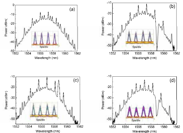
Figure 4. Spectra and waveforms of the 160 Gb/s data signal. (a) Original signal, (b) Carved spectrum before pilot insertion, (c) In-band pilot extraction, (d) In-band pilot extraction.
