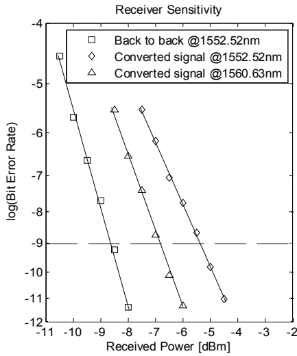
Figure 2. BER performance of 40 Gb/s wavelength conversion
