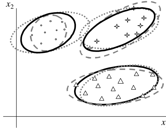
Figure 1. Geometric idea of the mixture covariance matrix.
