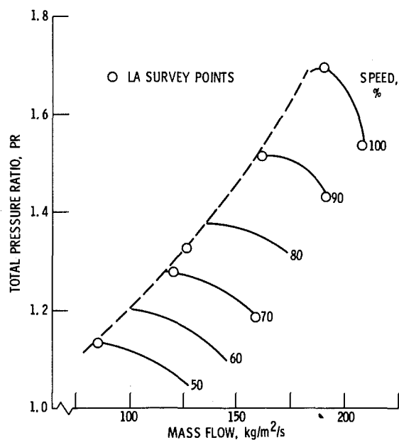
Fig. 2 Test compressor performance map
