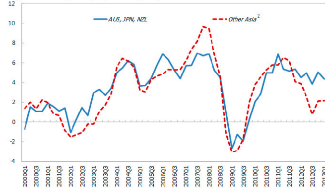
Figure 1: Non-FDI Inflows 1
