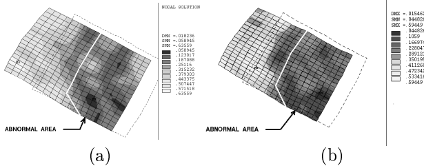
Figure 8: Resulting strain distribution for the skin motion experiment computed using (a) conventional approach and (b) proposed method.
