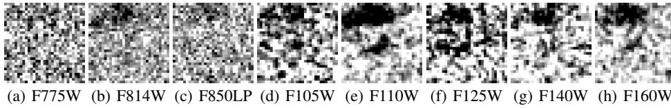
Fig. 2. 2.0'' \times 2.0'' thumbnail images of the population III galaxy candidate (centered in the image) in RXJ 1347. The images are from the eight CLASH filters covering the longest wavelengths, ranging between 6,500\text{\AA} and 17,000\text{\AA} . The Lyman-break is visible between F850LP and F105W since the object is observed in F105W but not in F850LP. The slight distortion from upper right to lower left that can be seen in the object (at least in some of the longer wavelength filters) could imply gravitational lensing with high magnification.
