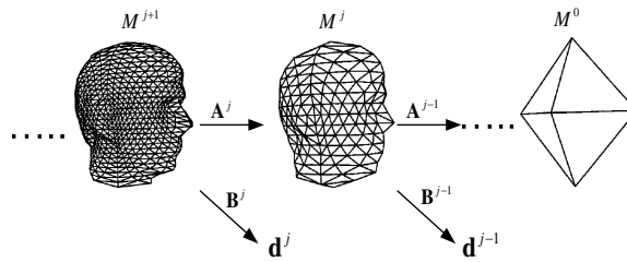
Fig. 2. Pictorial representation of the forward wavelet decomposition, (Lounsbery et al., 1997).
