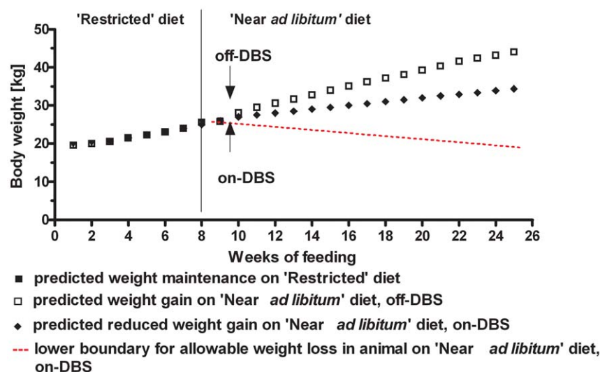
Figure 1. Predicted effect of hypothalamic DBS on weight gain in female Göttingen minipig. Study Design. We hypothesized that low frequency DBS would reduce the weight gain (◆) or induce a weight loss (red line), based on prior literature data on weight gain in the Göttingen minipig. Predicted values are also shown for weight changes (■) on a 'Restricted' diet (450 g/day) and for further weight gain (□) on a 'Near ad libitum ' diet (900 g/day).
