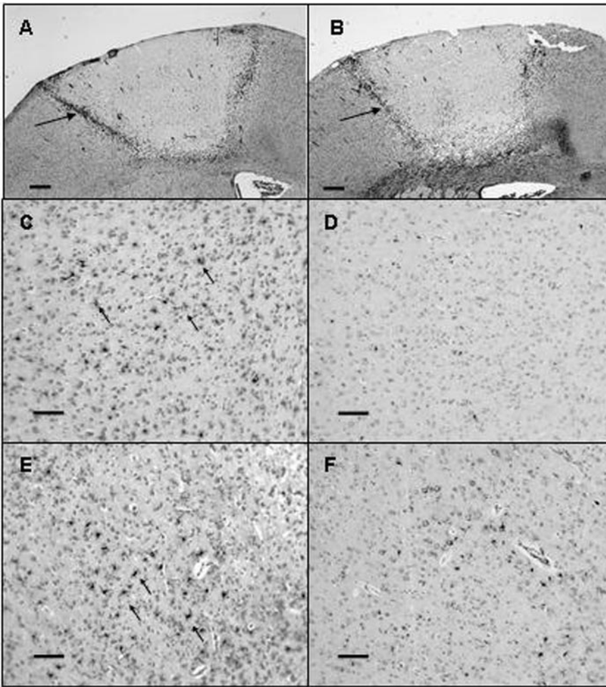
Fig. 2. Microglial and astroglial activation induced by photothrombosis. The left panel of the micrograph corresponds to untreated ischemic rats and the right panel to rats treated with 2,2'-dipyridyl (20 mg/kg, i.p., 15 min before and 1 h after photothrombosis). Five rats were examined in each group. Sections were stained with isolectin B4 (A and B) and glial fibrillary acidic protein (C to F) to visualize microglia and astrocytes, respectively, then they were counterstained with hematoxylin. The rim of microglial cells surrounding the infarcted area was found similar between the two groups of rats (A and B, see arrow). Astroglial activation was visible outside and close to the infarcted area (C and D) as well as in the parietal cortex (E and F) and was found in both cases to be of a lesser extent in treated rats. Scale bars = 400 \mu\text{m} (A and B), 100 \mu\text{m} (C to F).
