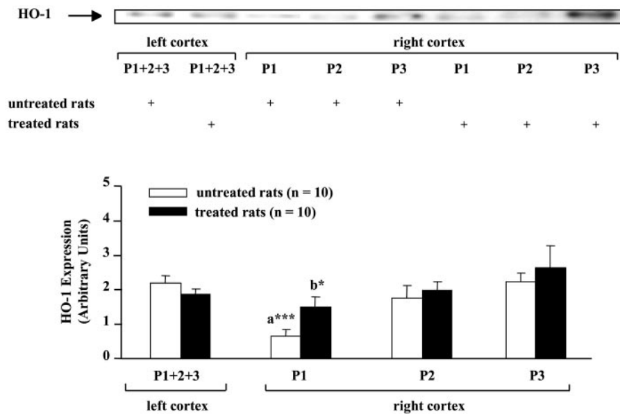
Fig. 8. Effect of 2,2'-dipyridyl on photothrombosis-induced changes in HO-1. See Fig. 7 for legend. *, p < 0.05 ; ***, p < 0.001 ; a, versus left cortex; b, versus untreated rats.
