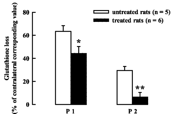
Fig. 6. Effect of 2,2'-dipyridyl on photothrombosis-induced glutathione loss. Glutathione levels were measured in cortex contralateral and ipsilateral to irradiation. Bars show glutathione loss in P1 and P2 samples expressed as percentage of contralateral corresponding values. 2,2'-Dipyridyl (20 mg/kg, i.p.) or vehicle was given 15 min before and 1 h after photothrombosis. Bars are means \pm S.E.M. n = number of rats. See Fig. 3 for details of tissue sampling. *, p < 0.05 and **, p < 0.01 versus untreated rats.
