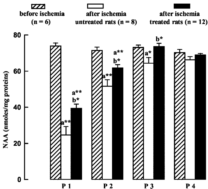
Fig. 4. Effect of 2,2'-dipyridyl on photothrombosis-induced NAA loss. NAA levels were measured before ischemia and at day 1 after ischemia in the irradiated cortex. Ischemic rats received 20 mg/kg 2,2'-dipyridyl (treated rats) or vehicle (untreated rats) 15 min before and 1 h after photothrombosis. P1, P2, P3, and P4 samples were collected as indicated in Fig. 3. Bars are means \pm S.E.M. n = number of rats; *, p < 0.05 ; **, p < 0.01 ; a, versus before ischemia; b, versus untreated rats.
