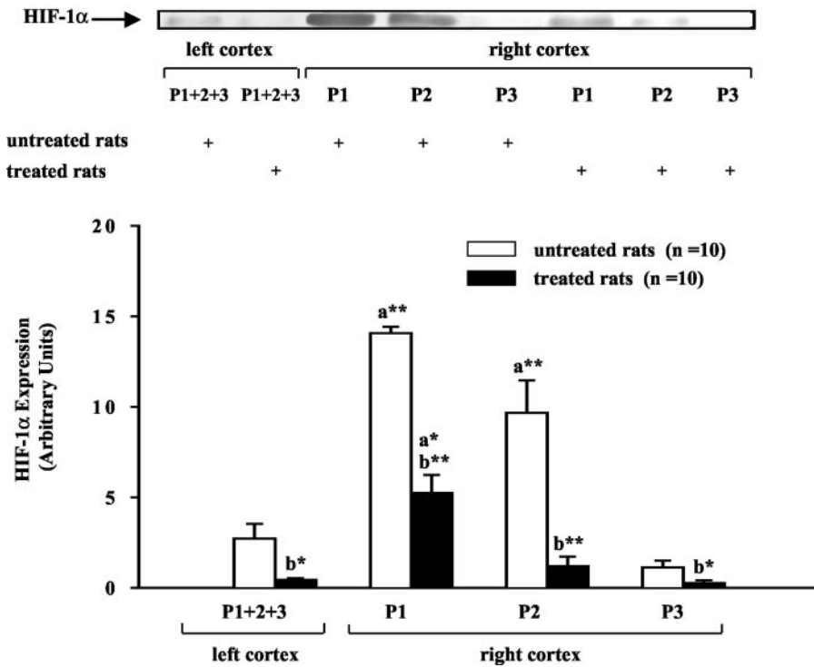
Fig. 7. Effect of 2,2'-dipyridyl on photothrombosis-induced changes in HIF-1 \alpha . HIF-1 \alpha protein expression was examined in P1, P2, and P3 samples collected from the lesioned cortex (right cortex) and the unlesioned contralateral cortex (left cortex) on day 1 after photothrombosis. The values in the left cortex were pooled. 2,2'-Dipyridyl (20 mg/kg) or vehicle was injected (i.p.) 15 min before and 1 h after photothrombosis initiation. Bars are means \pm S.E.M. n = number of rats; *, p < 0.05 ; **, p < 0.01 ; a, versus left cortex; b, versus untreated rats.
