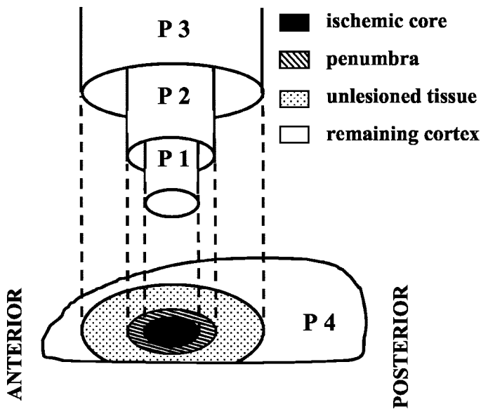
Fig. 3. Three concentric cortical samples (P1, P2, and P3) were collected using punches with increasing internal diameter (2.8, 4.6, and 9.5 mm, respectively). P1 corresponded to the ischemic core (unsalvageable tissue), P2 to the penumbra (salvageable tissue), and P3 to unlesioned tissue. P4 corresponded to the remaining cortex. P1 was centered on the infarct that was macroscopically readily observable (petechial hemorrhages).
