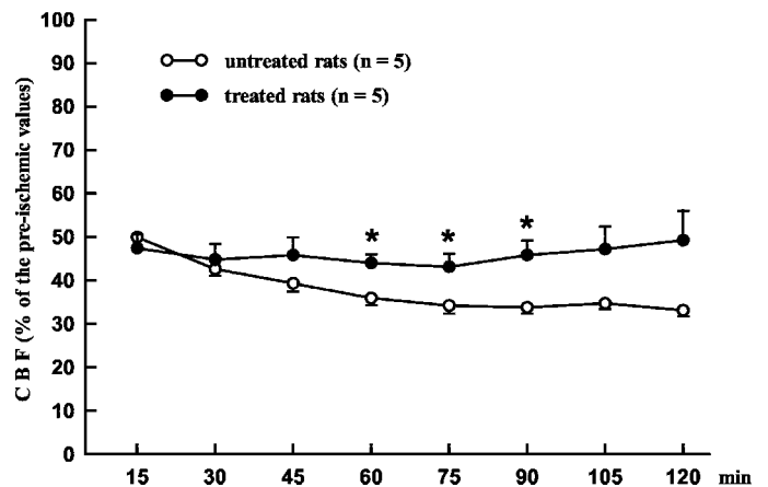
Fig. 5. Effect of 2,2'-dipyridyl on the time course of CBF after photothrombosis. Values are expressed as percentage of preischemic contralateral CBF, which was recorded before treatment initiation. 2,2'-Dipyridyl (20 mg/kg, i.p.) or vehicle was given 15 min before and 1 h after photothrombosis. Values are expressed as means \pm S.E.M. n = number of rats; *, p < 0.05 versus untreated rats.
