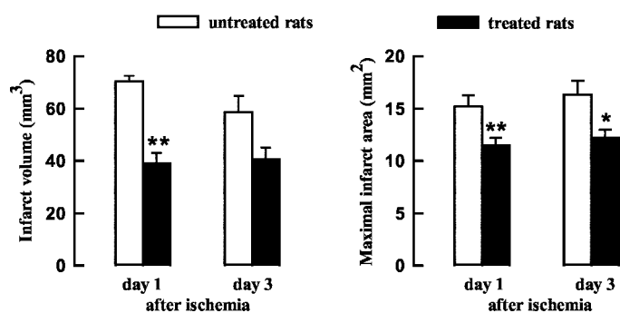
Fig. 1. Effect of 2,2'-dipyridyl on infarct volume ( \text{mm}^3 ) and maximal infarct area ( \text{mm}^2 ). 2,2'-Dipyridyl (20 mg/kg, i.p.) was given 15 min before and 1 h after photothrombosis. Bars are means \pm S.E.M. from five to six rats. *, p < 0.05 and **, p < 0.01 versus untreated rats.
