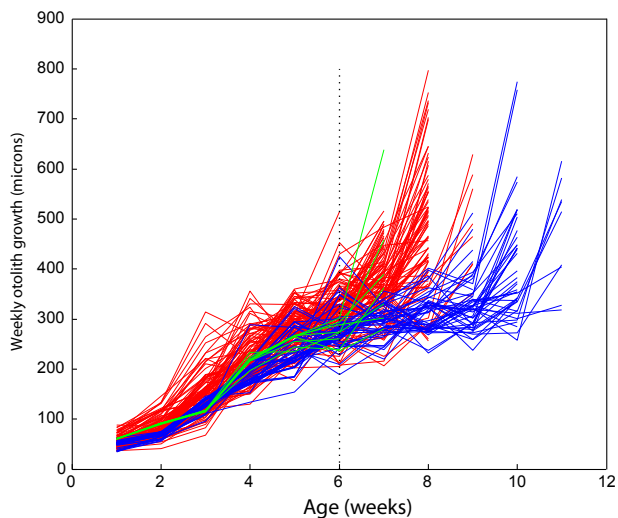
Fig. 6. Individual bluefish otolith growth used to fit all models. Spring cohort is represented in red, summer cohort is blue and the autumn cohort is green. The dashed line represents the mean age of estuarine recruitment of for bluefish.
