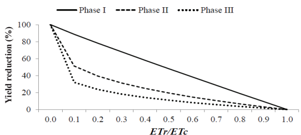
Figure 2. Yield reduction as a function of the ET_r/ETc ratio, based on the Jensen (1968) model, using statistically adjusted coefficients in the development phases I, II and III (Paranavaí, Paraná State, Brazil).
