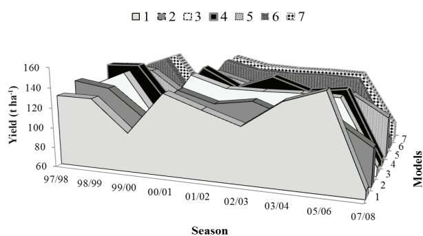
Figure 1. Real and estimated ratoon sugarcane yield from the 1997/1998 to the 2007/2008 season (Paranavaí, Paraná State, Brazil). 1 - Real yield; 2-7 - Estimated yield with models; 2 - Howell & Hiler (1975); 3 - Jensen (1968); 4 - Minhas et al. (1974); 5 - Doorenbos & Kassam (1979); 6 - Stewart et al. (1976) proposed by Doorenbos & Kassam (1979); 7 - Rao et al. (1988).
