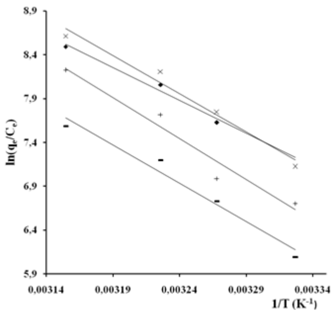
Fig. 6 Plot of \ln(q_e/C_e) vs 1/T for chlordiazeopoxide ( \Delta H_{ads} > 50 kJ/mol) on NB (x) BDH (+) Merck (x) M (-).
