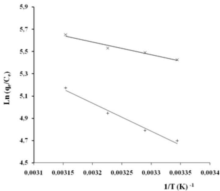
Fig. 7 Plot of \ln(q_e/C_e) vs 1/T for diazepam ( \Delta H < 20 kJ/mol) on BDH(+) Merk (x).
