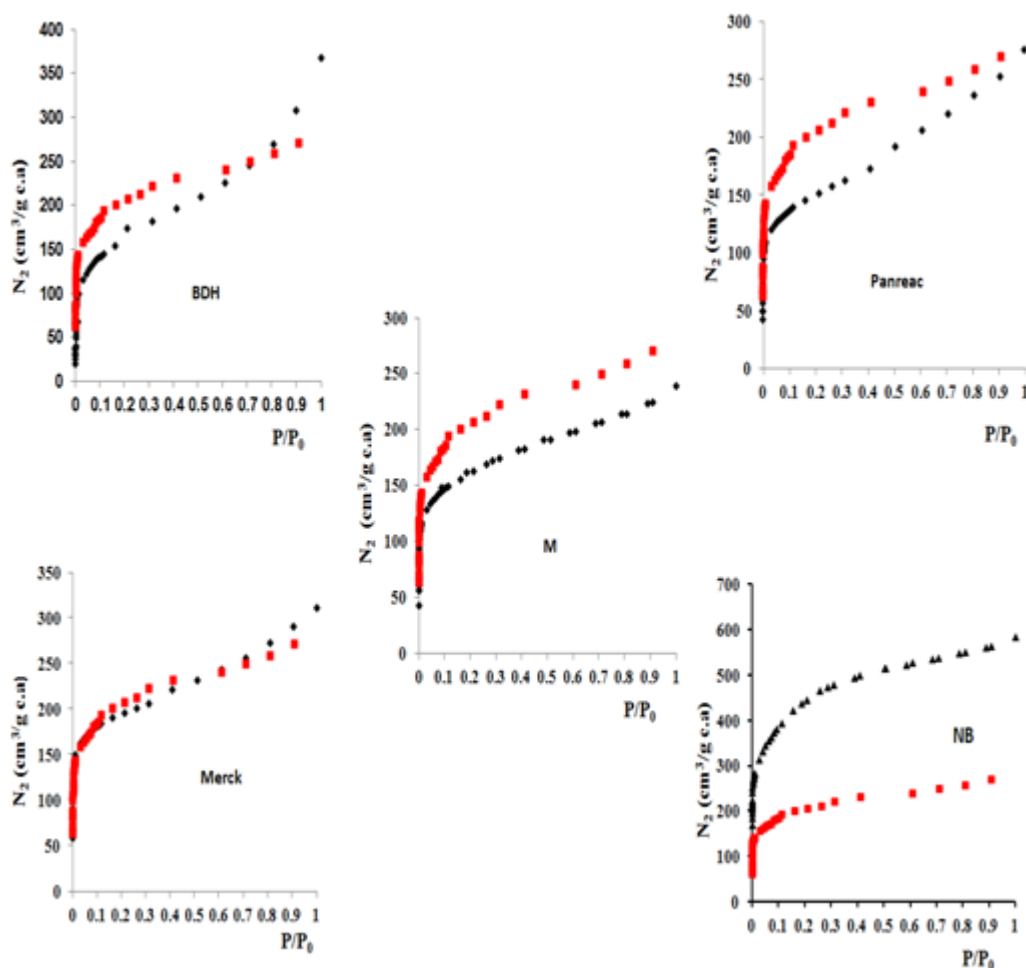
Fig.3 N 2 adsorption isotherms at T = 77 K, ML (■).
