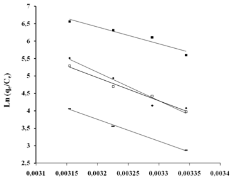
Fig. 8 Plot of \ln(q_e/C_e) vs 1/T for diazepam ( \Delta H > 20 kJ/mol) on (NB (♦) ML 4 (■) M (-) Panreac (□)
