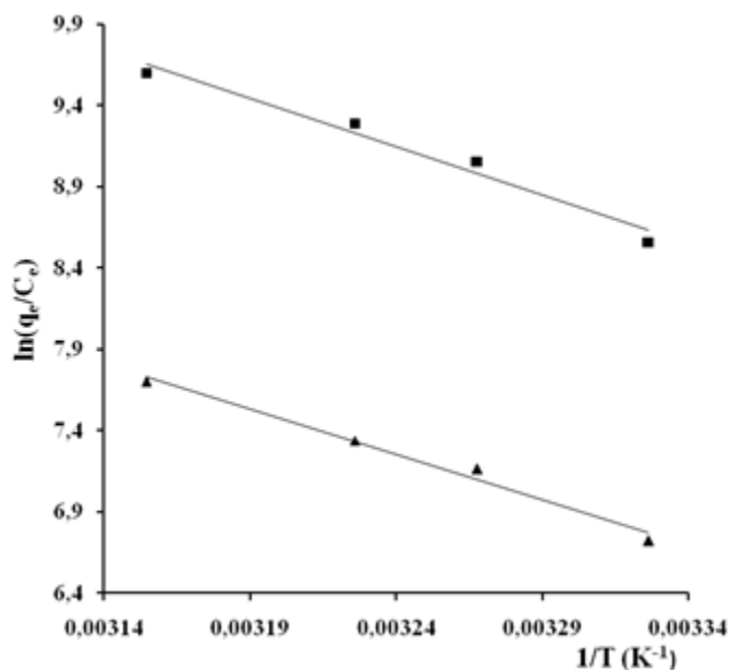
Fig. 5 Plot of \ln(q_e/C_e) vs 1/T for chlordizepoxide ( \Delta H_{ads} < 50 kJ/mol) on P (■) ML (▲).
