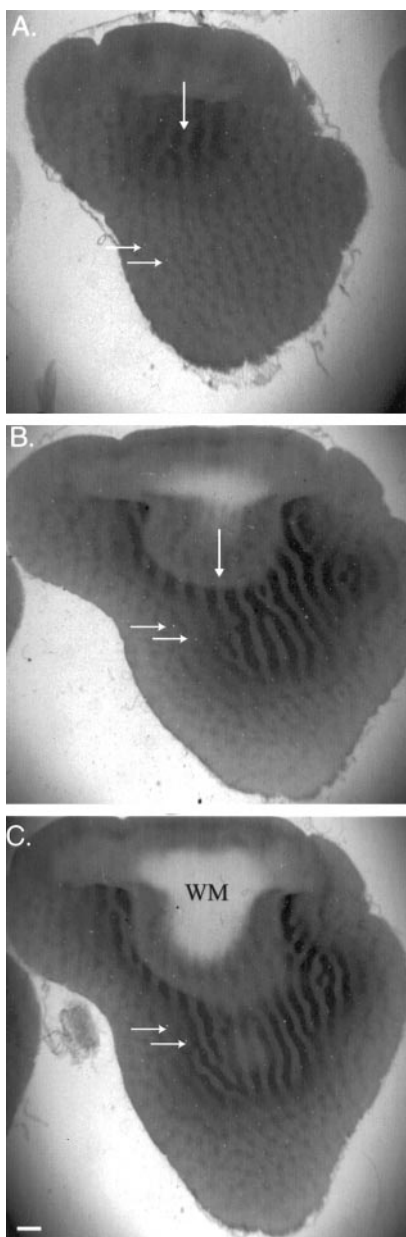
FIGURE 8. Tangential serial sections stained for COR through the ipsilateral V1 cortex of a monkey with experimental glaucoma of the right eye. Vertical arrow: CO-rich ODC in layer 4C, which has input from the normal left eye. The adjacent CO-poor ODC has input from the glaucomatous right eye. Horizontal arrows: same blood vessels, which could serve as fiducial alignment marks. The alternating rows of CO-rich blobs in layers 2 and 3, which lie directly above the ODC of layer 4C, can be seen in (A). WM, white matter. Bar, 1 mm.
