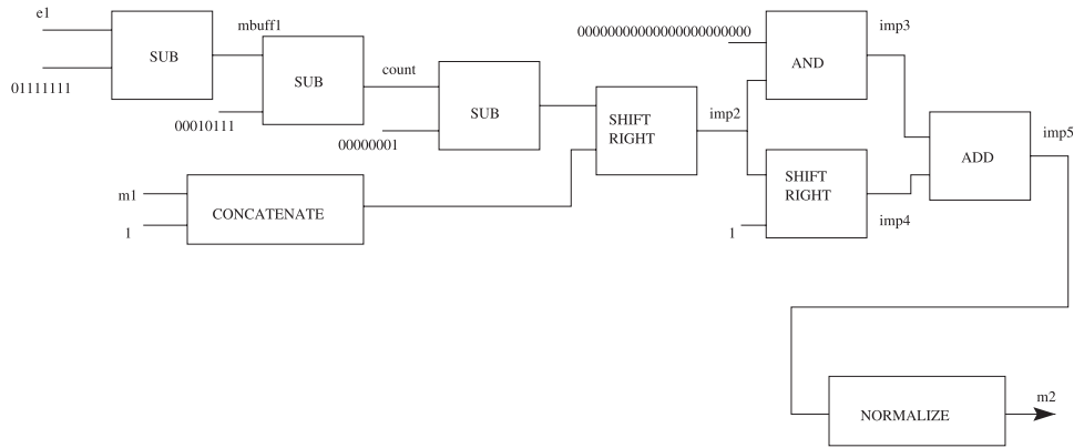
FIGURE A3. Round to nearest integer block diagram.
