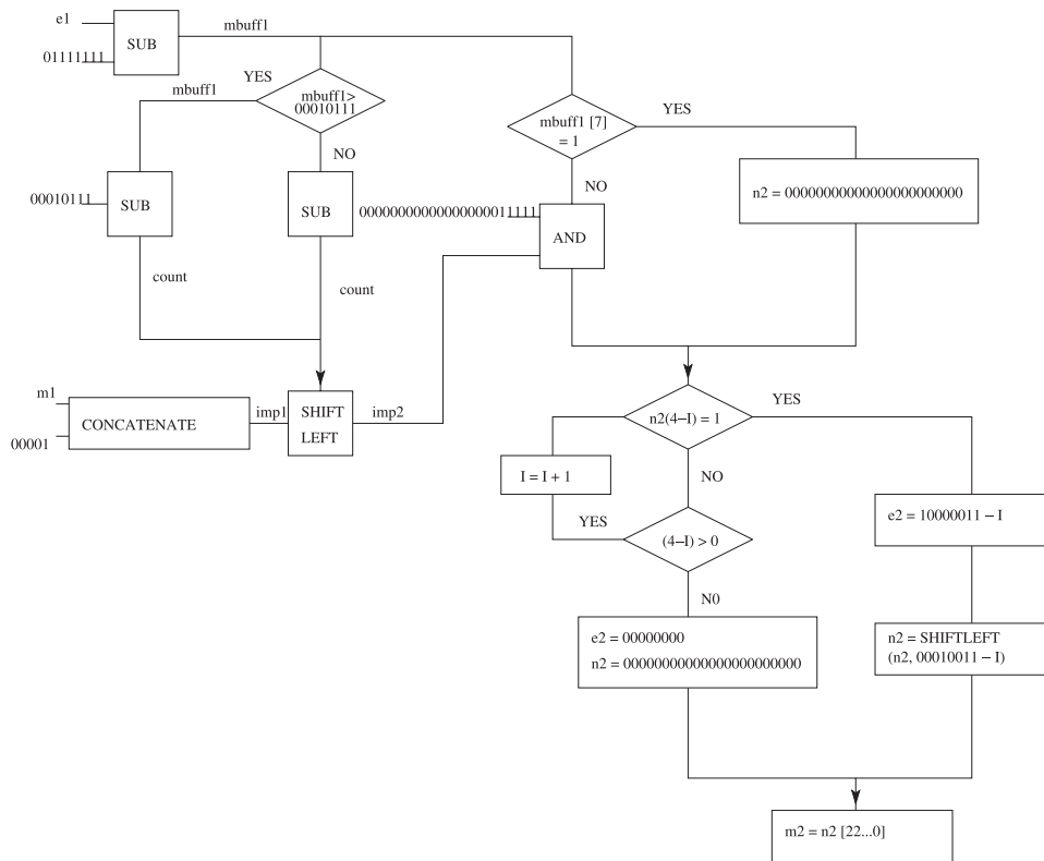
FIGURE A4. Modulo-32 block diagram.
