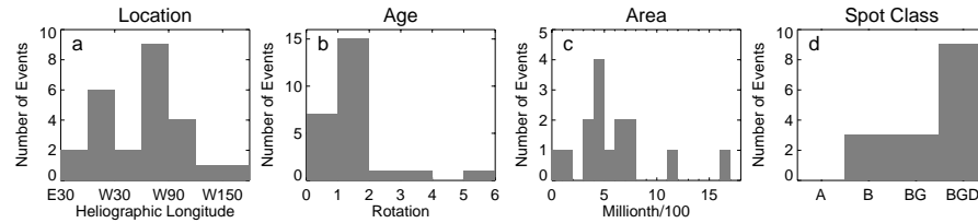
Fig. 1. Characteristics of the active regions linked to major SEP events
